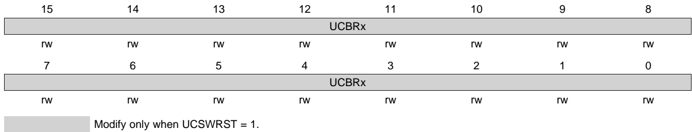
Figure 38-6. UCxBRW Register
