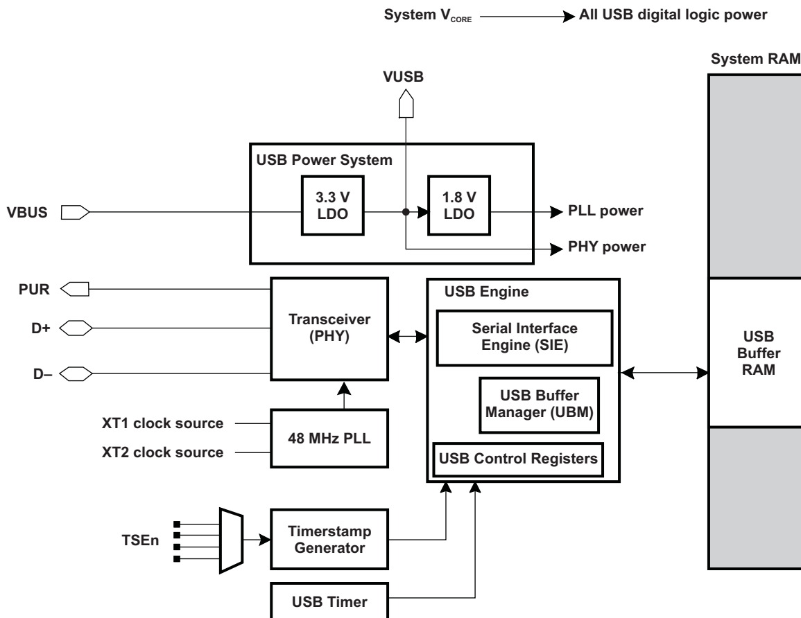
Figure 40-1. USB Block Diagram
