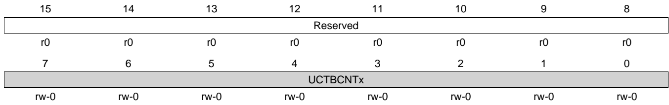
Figure 39-21. UCBxTBCNT Register
