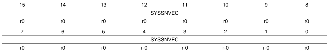
Figure 1-19. SYSSNIV Register
