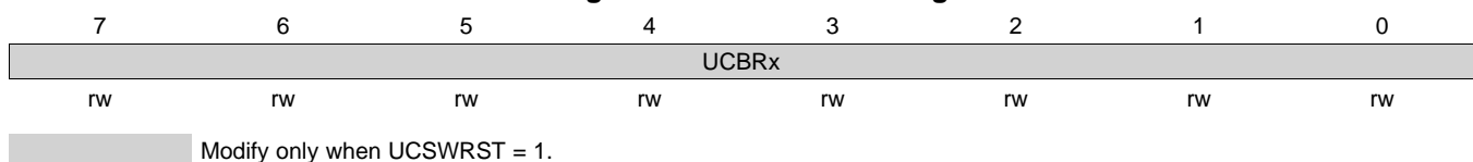
Figure 34-15. UCxBR1 Register
