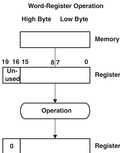
Figure 6-12. Word-Register Operation
