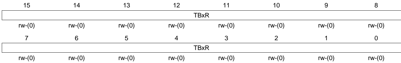
Figure 18-17. TBxR Register
