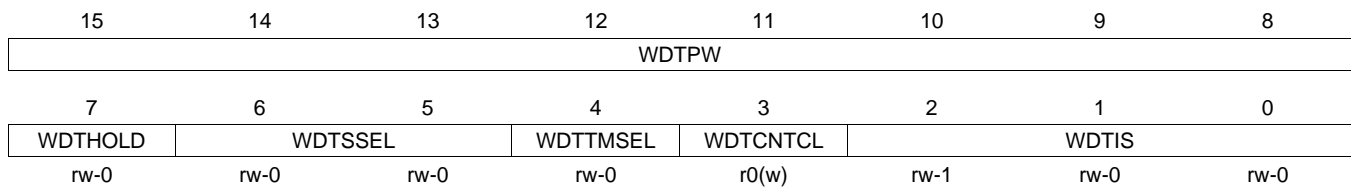
Figure 16-2. WDTCTL Register
