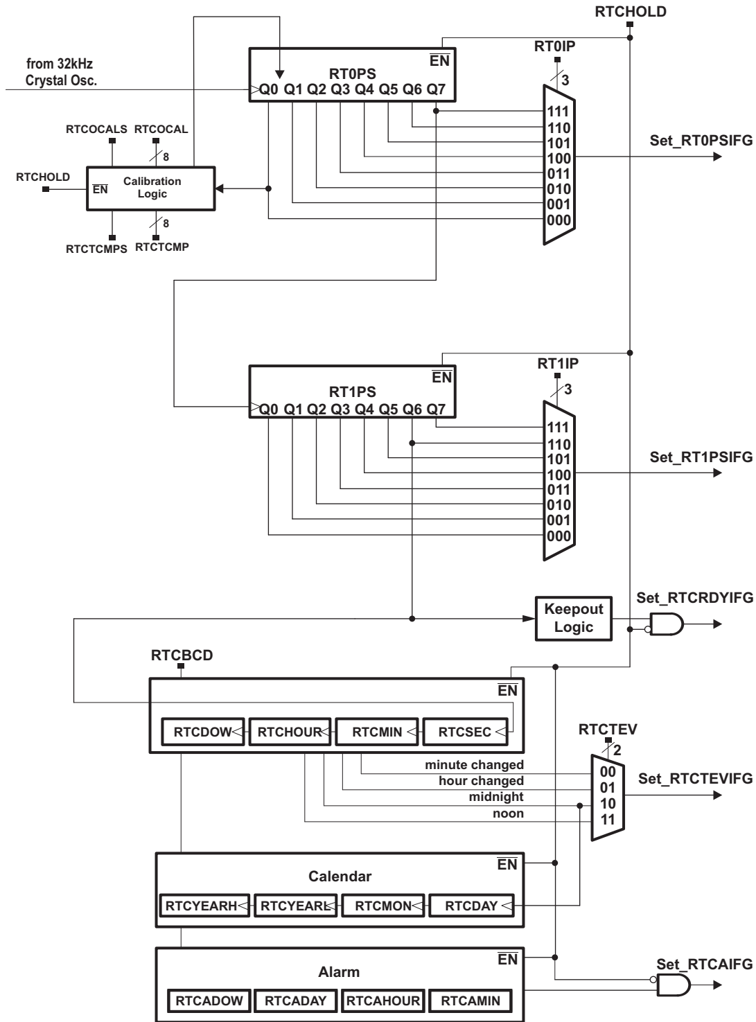
Figure 24-1. RTC_C Block Diagram
