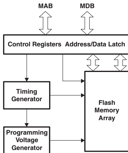
Figure 7-1. Flash Memory Module Block Diagram
