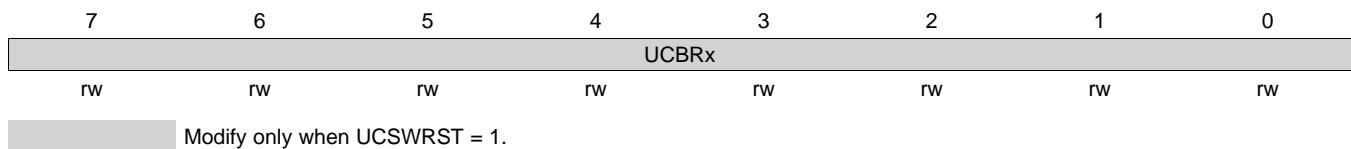
Figure 34-14. UCxBR0 Register
