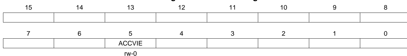
Figure 7-17. SFRIE1 Register
