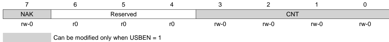
Figure 40-18. USBOEPBCNT_0 Register
