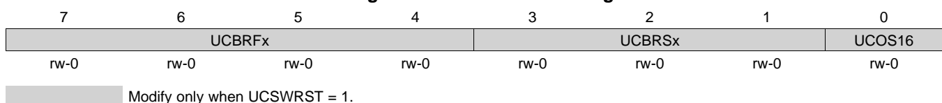
Figure 34-16. UCxMCTL Register
