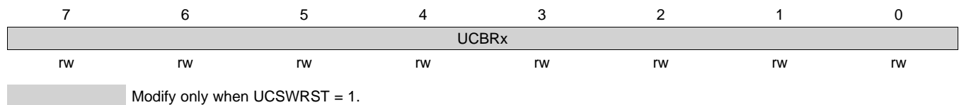
Figure 36-19. UCBxBR0 Register
