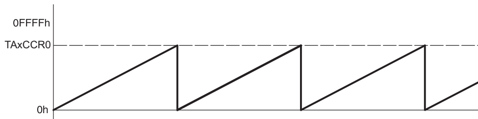
Figure 17-2. Up Mode
