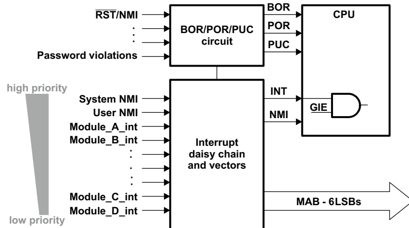
Figure 1-2. Interrupt Priority
