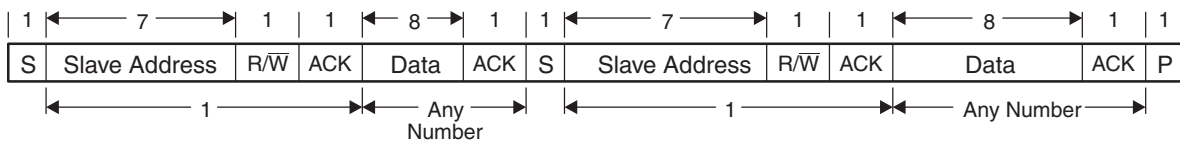
Figure 39-7. I 2 C Module Addressing Format With Repeated START Condition
