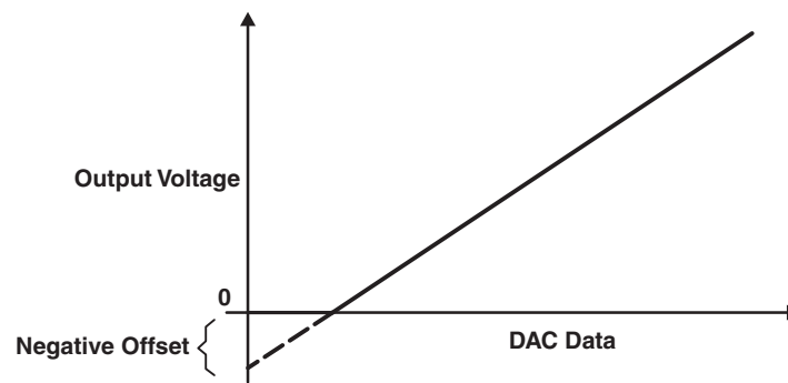
Figure 30-5. Negative Offset
