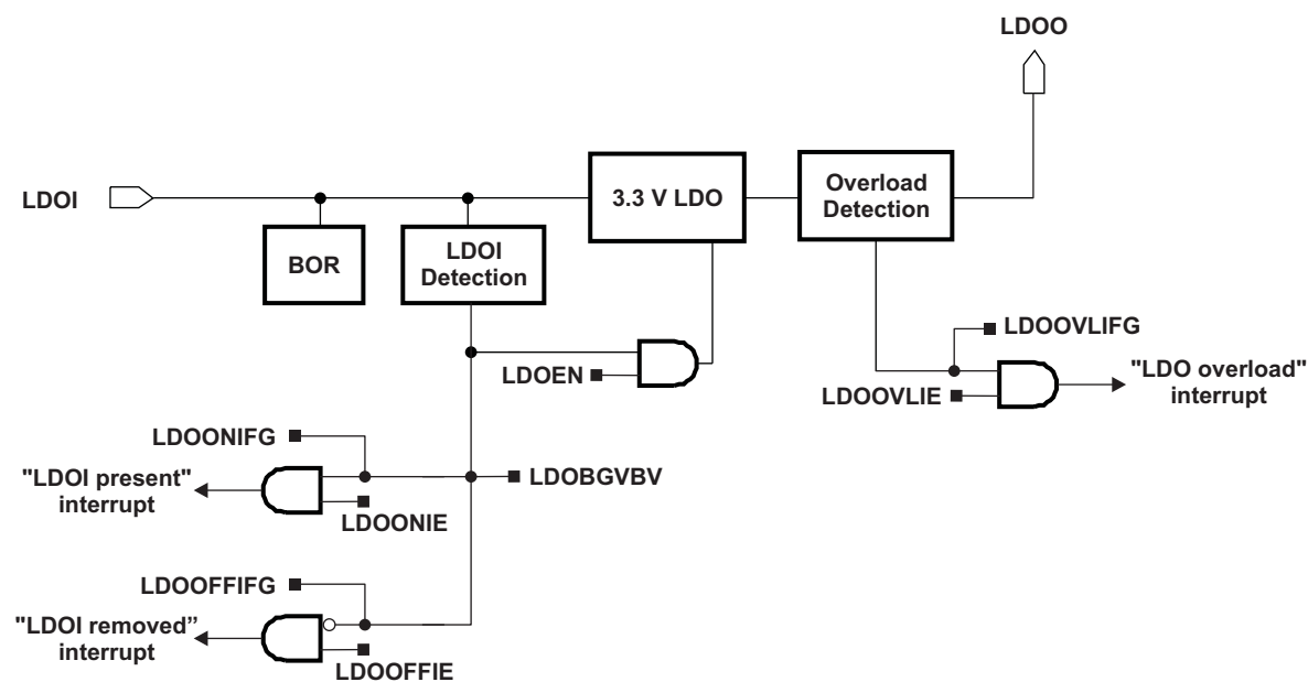
Figure 41-1. LDO Block Diagram
