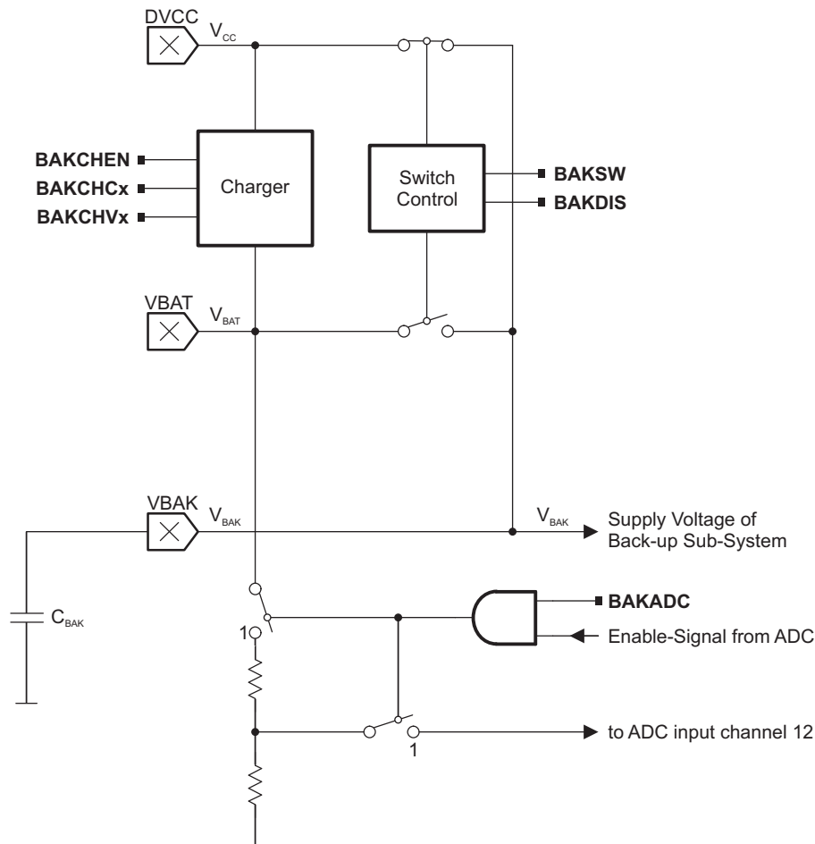
Figure 3-1. Battery Backup Switch Overview
