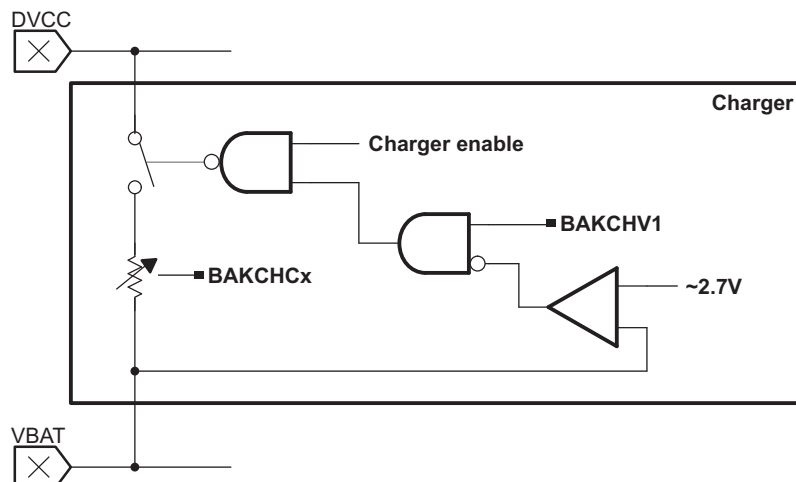
Figure 3-2. Charger Block Diagram
