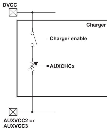
Figure 4-8. Charger Block Diagram
