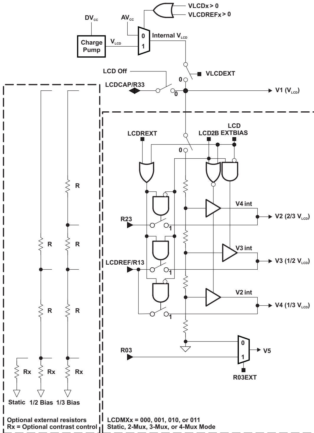
Figure 33-4. Bias Generation
