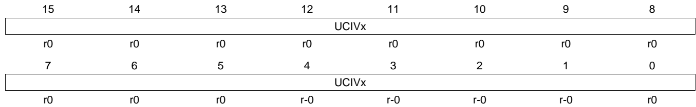
Figure 35-15. UCAXIV Register
