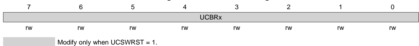
Figure 36-20. UCBxBR1 Register
