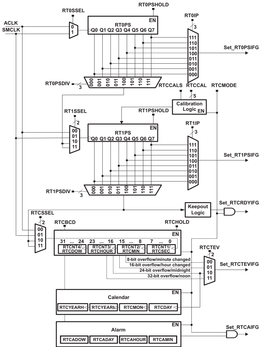
Figure 22-1. RTC_A
